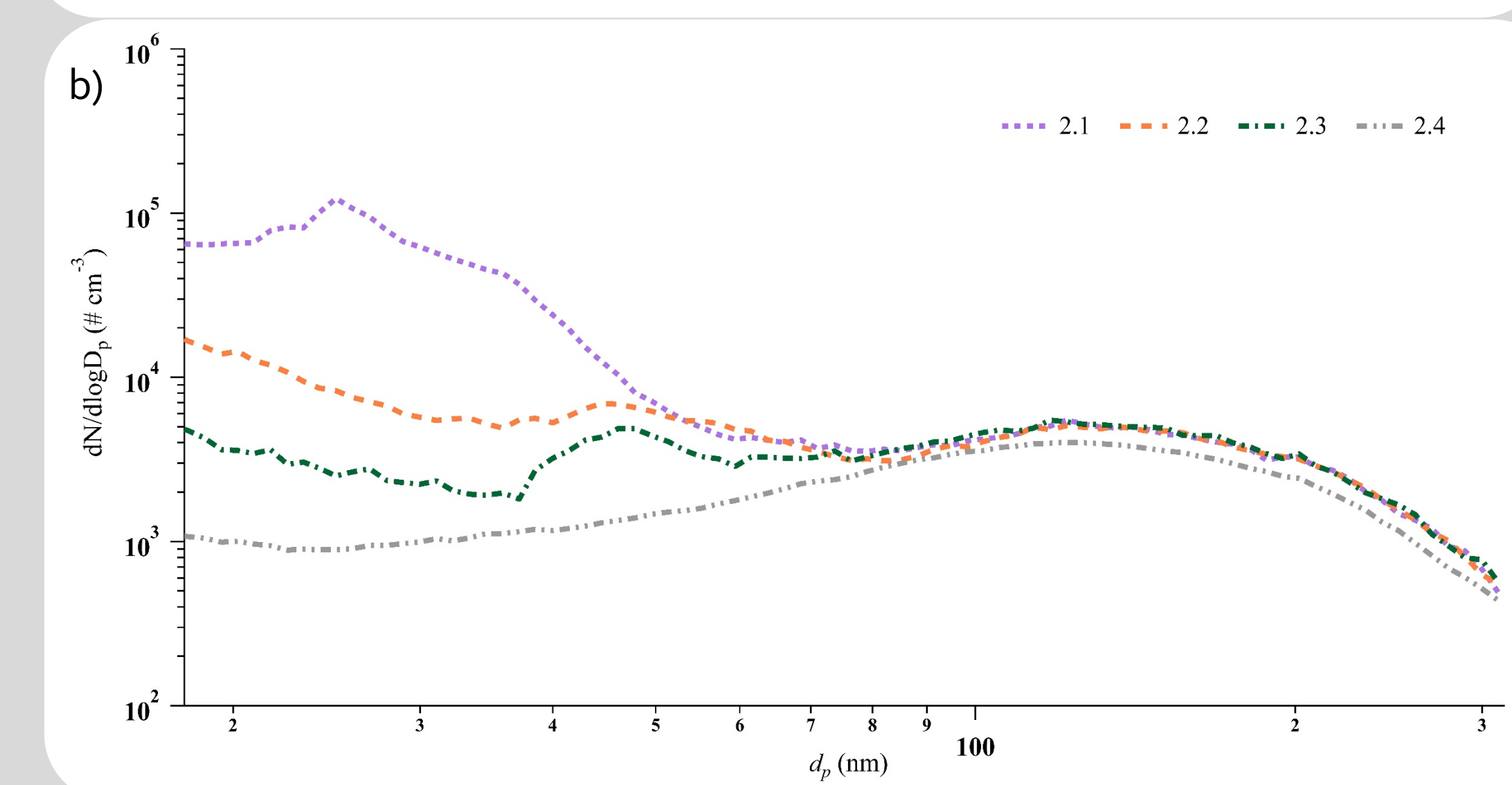
Figure 3. Mean aerosol particle size distribution during the different phases of: a) process 1: printing 3DP mould; b) process 2: melting and pouring.
