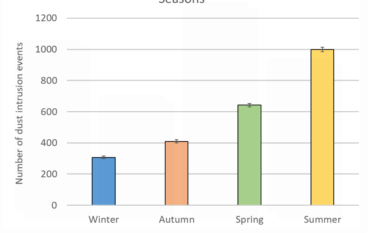
Fig. 5. Number of Saharan dust intrusion events by seasons in the Iberian Peninsula between 2005 and 2020.
