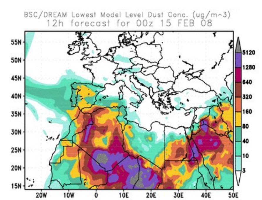
Fig. 14. Dust concentration (µg / m 3 ) for February 15, 2008 obtained from the BSC / DREAM model.
