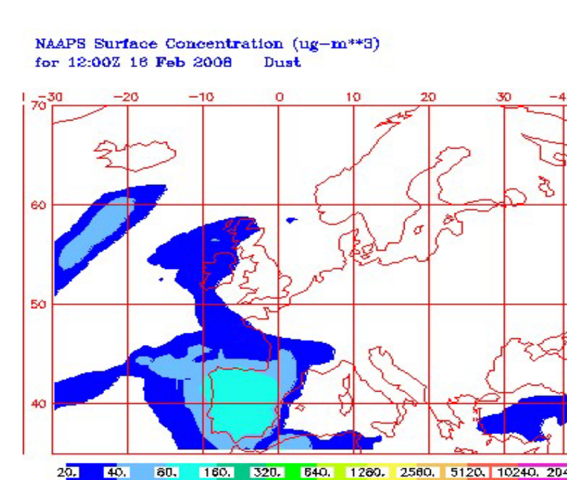
Fig. 13. Dust concentration (µg / m 3 ) for February 16, 2008, obtained from the NAAPs model.
