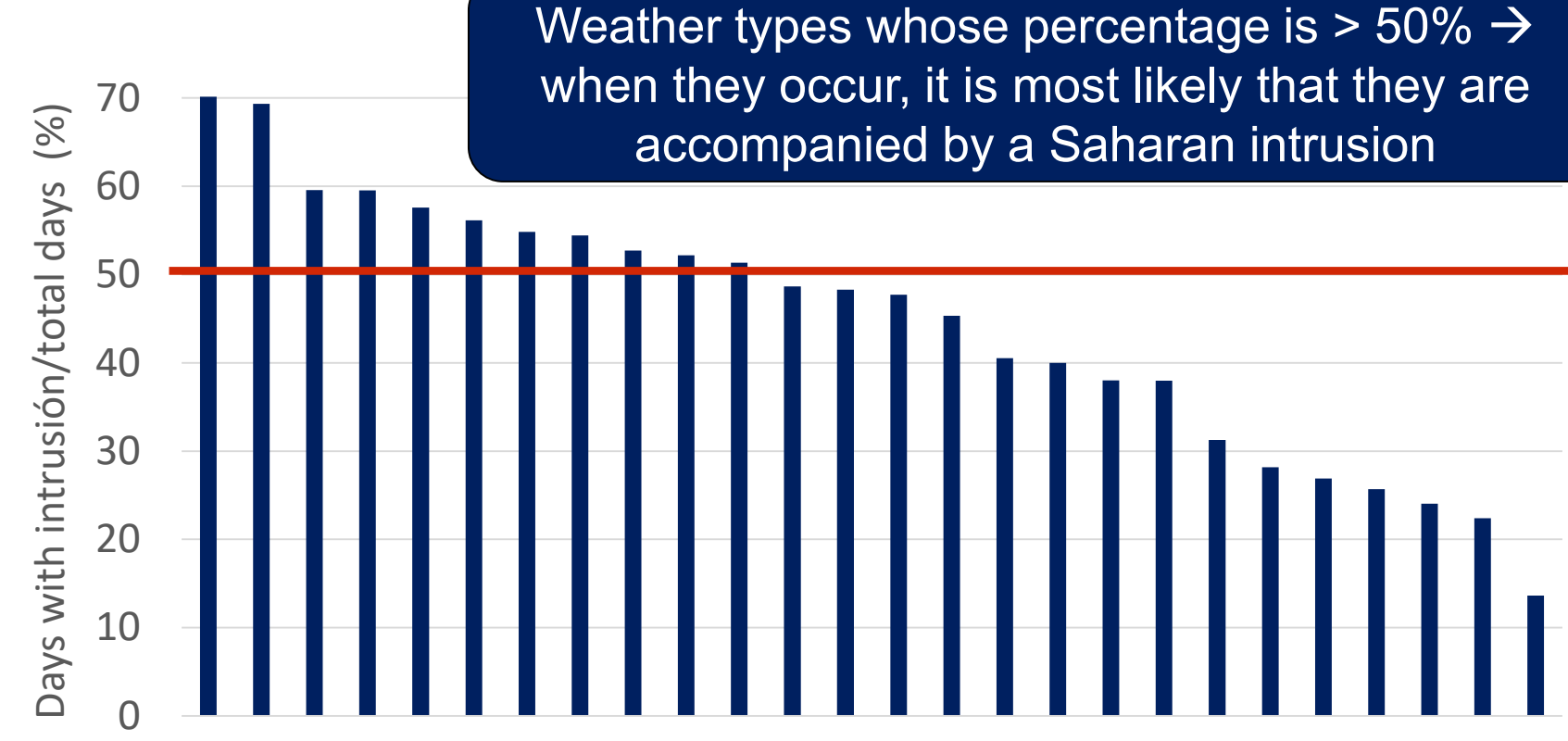
Fig. 4. For each weather type, ratio between days with Saharan dust intrusion and total days during the study period.
